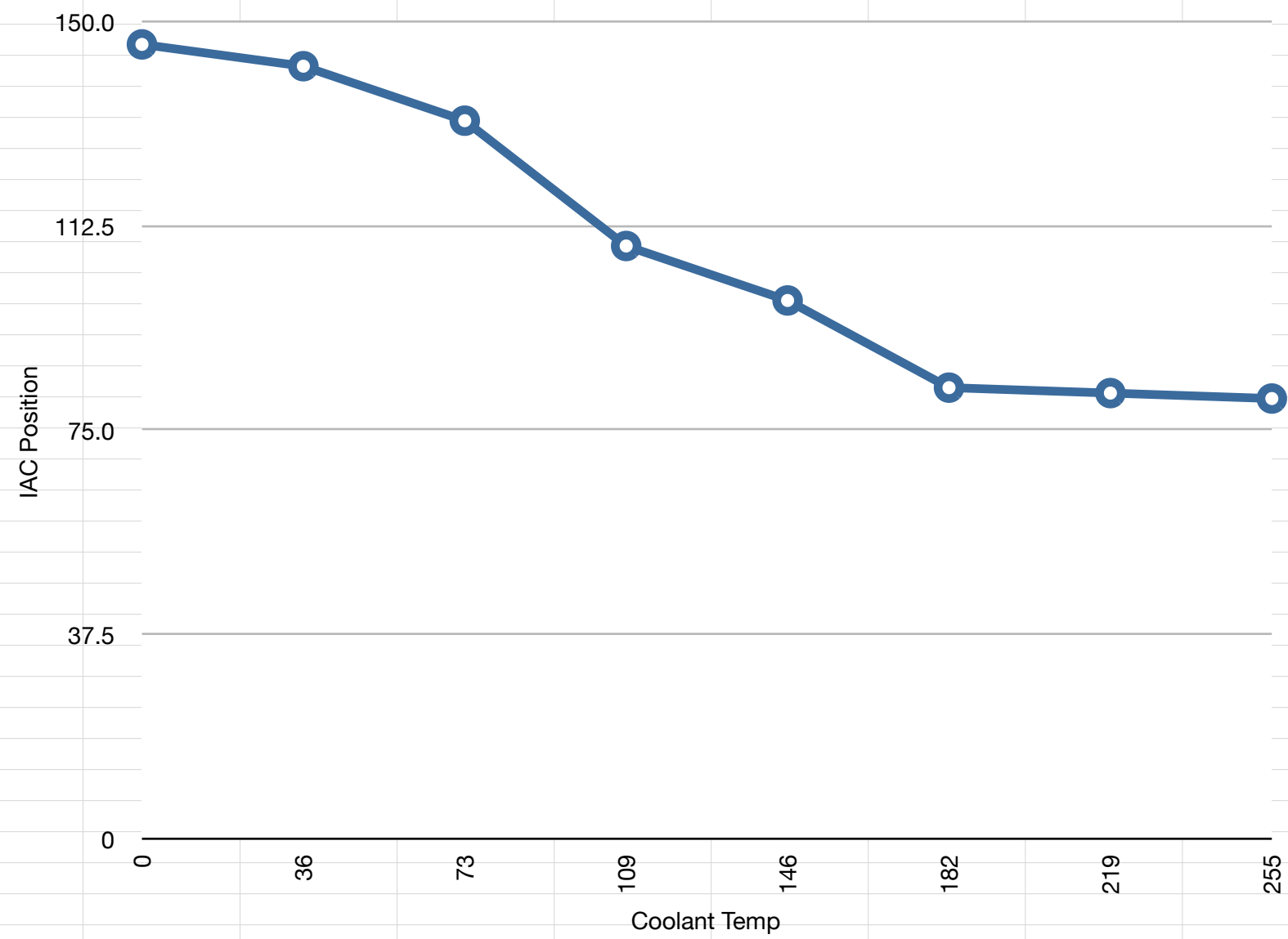
IAC Start Position vs Coolant Temp
